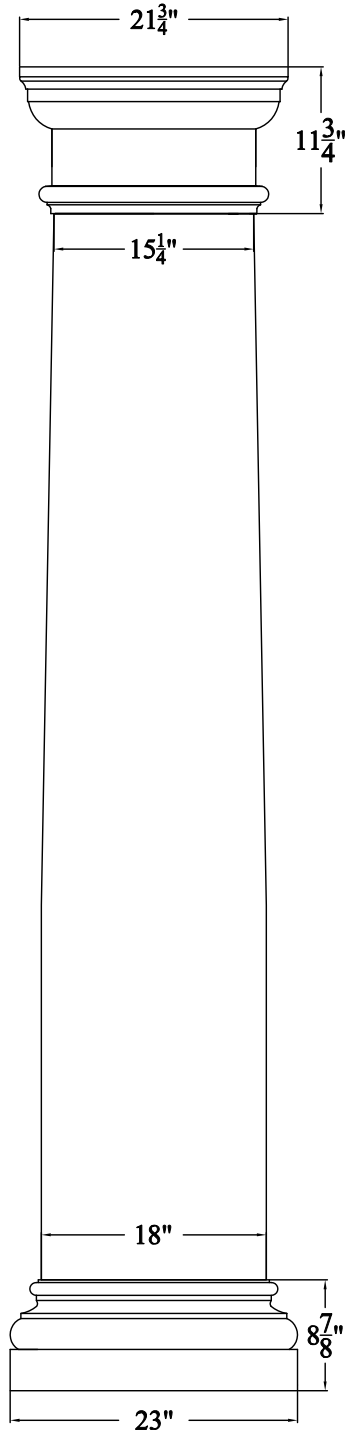
COL18B
