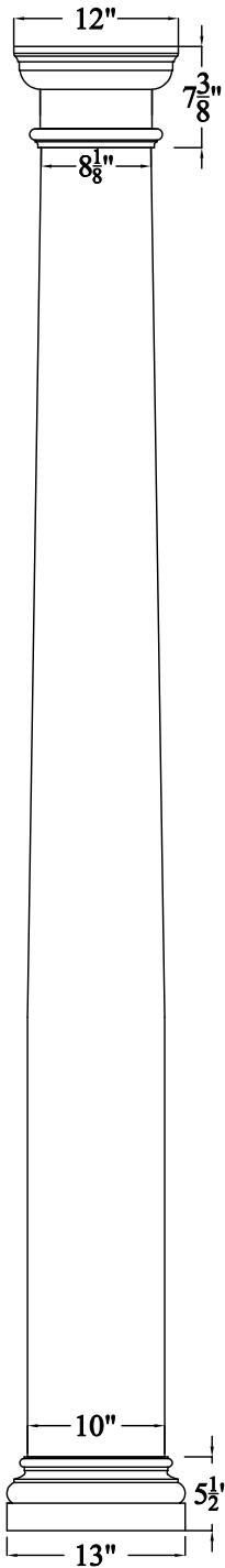
COL10B
