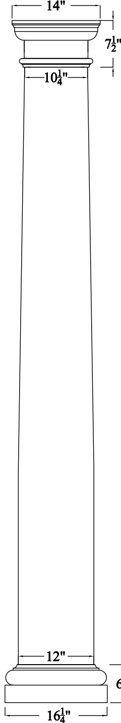
COL12A
