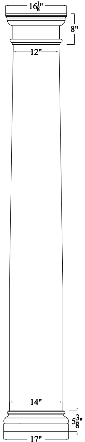
COL14B
