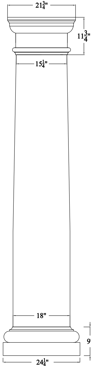
COL18A
