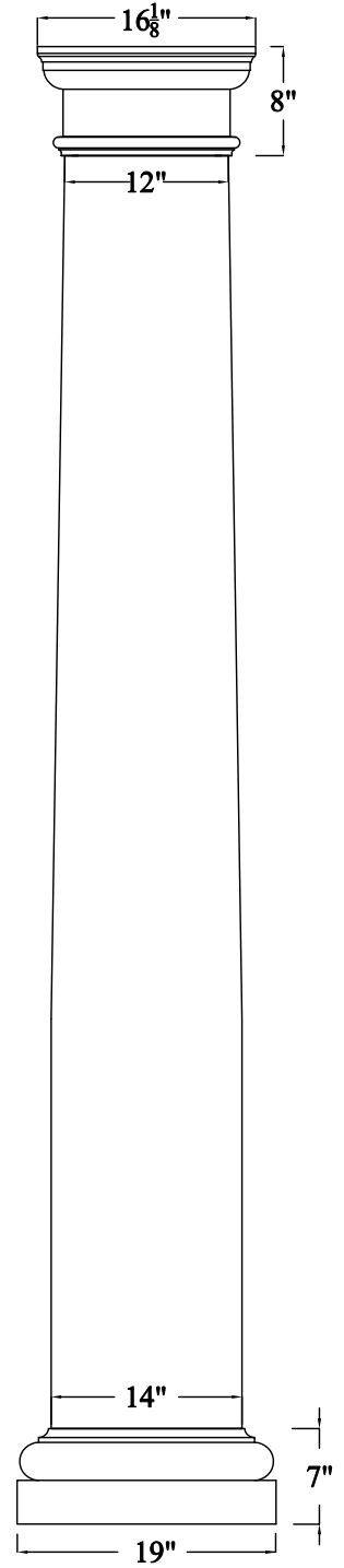
COL14A
