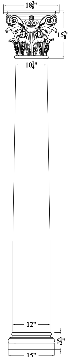
COL12C
